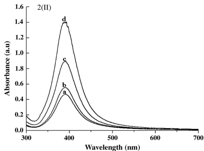
Figure 2 (I) TEM image of silver NPs and 2(II) absorbance spectra of silver NPs. Conditions: Silver NPs 1 \times 10^{-4} \text{ M} , 2 \times 10^{-4} \text{ M} , 3 \times 10^{-4} \text{ M} , 4 \times 10^{-4} \text{ M} .
