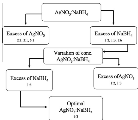
Scheme 1 Schematic for the preparation of silver NPs.
