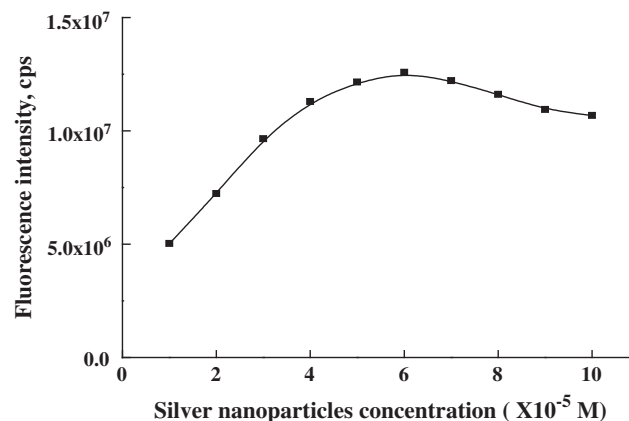
Figure 3 Effect of NPs concentration on the FL intensity. Conditions: FEX 1.5 \times 10^{-5} \text{ M} .
