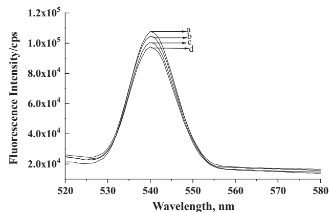
Figure 4 FL emission spectra (excitation at 391 nm) of silver NPs at 541 nm in the absence (a) and in the presence (b, c, d) of FEX. Conditions: FEX (b) 1.5 \times 10^{-6} , (c) 3.3 \times 10^{-6} and (d) 1.6 \times 10^{-5} M; (a) Silver NPs 6 \times 10^{-5} M.
